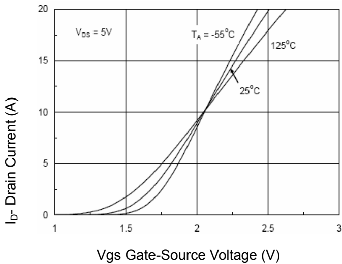
Figure 1 Output Characteristics
