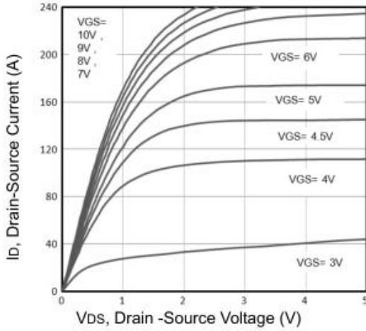
Fig 1: Output Characteristics
