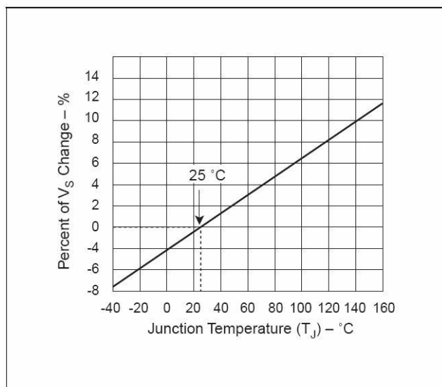
Figure Normalized V_S Change versus Junction Temperature
